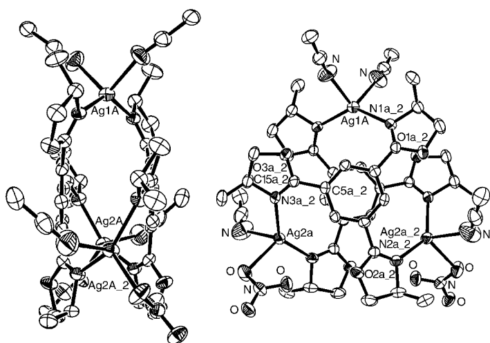
Figure 1. Structure of (M)-[\text{Ag}_3\text{L}_2^{*\text{Me}(S)}](\text{CH}_3\text{CN})_4(\text{NO}_3)_2]^+ in the solid state (ORTEP representations). Side view (left) and top view along pseudo- C_3 symmetric helical axis (right). All hydrogen atoms are omitted for clarity, only the heteroatoms of the upper \text{L}^{*\text{Me}} ligand, the nitrate, and the acetonitrile ligands are indicated in the top view. Selected torsional angles [\circ] (bond lengths [\text{\AA}] ; bond angles [\circ] ) for C5a_2, C15a_2, N3a_2, Ag2a: -7.9 (1.480, 1.263, 2.243; 126.99, 131.69).
