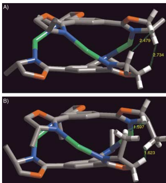
Figure 2. A) Crystal structure of (M)-[\text{Ag}_3\text{L}_2^{*\text{Me}(S)}]^{3+} and B) model structure of (M)-[\text{Ag}_3\text{L}_2^{*\text{Me}(R)}]^{3+} . All hydrogen atoms except those at interacting sites are omitted for clarity. Atom color code: C (gray), O (red), N (blue), Ag (green), H (white). Both views were generated with the Cerius2 program.
